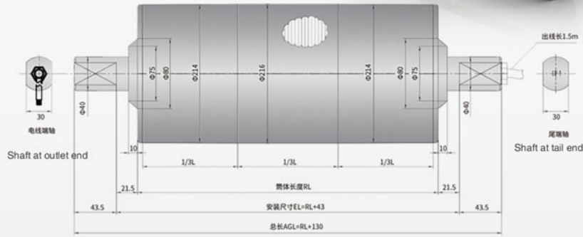
Dimensions of DM216 electric roller
