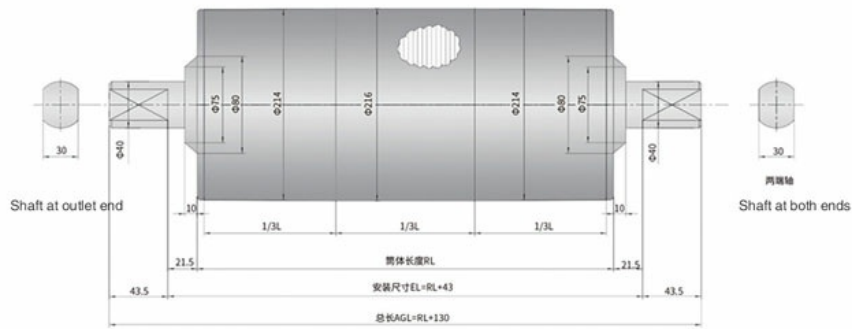
Dimension drawing of DM165 driven roller
