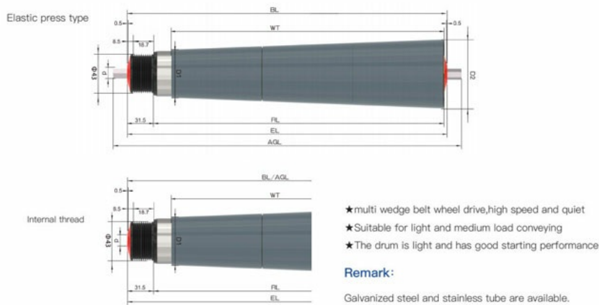
Plastic Poly-V Belt Conveyor Roller Tapered Drum For Curved Conveyor
